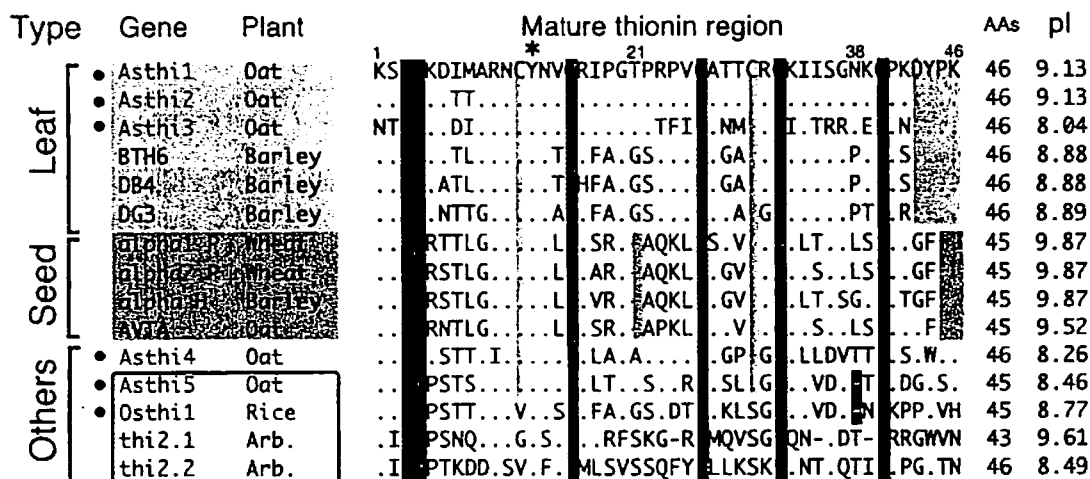
Fig. 2. Characteristics of oat leaf-specific thionin genes. A comparison of the mature thionin region of representative plant thionins. Leaf-type (shown in green), seed-type (orange) and other thionins were classified using the neighbor-joining method (Saitou and Nei 1987) by GENETIX 9.0 (Software Development Co., Tokyo). Conserved cysteine residues are shaded in lighter purple or blue. The conserved thirteenth tyrosine residue is marked with an asterisk. The sequences are from BTH6 (Holtorf et al. 1995), DB4 and DG3 (Bohlmann and Apel 1987), \alpha 1- and \alpha 2-purothionin (Mak and Jones 1976), \alpha -hordothionin (Rodriguez et al. 1988), and thi2.1 and thi2.2 (Epple et al. 1995). The sequences of Asthi1 through Asthi5 (GenBank accession numbers AB072338 to AB072342) and Osthi1 (accession number AB072337) are from the present study. AAs = number of amino acids. The calculated isoelectric point is given on the right.
